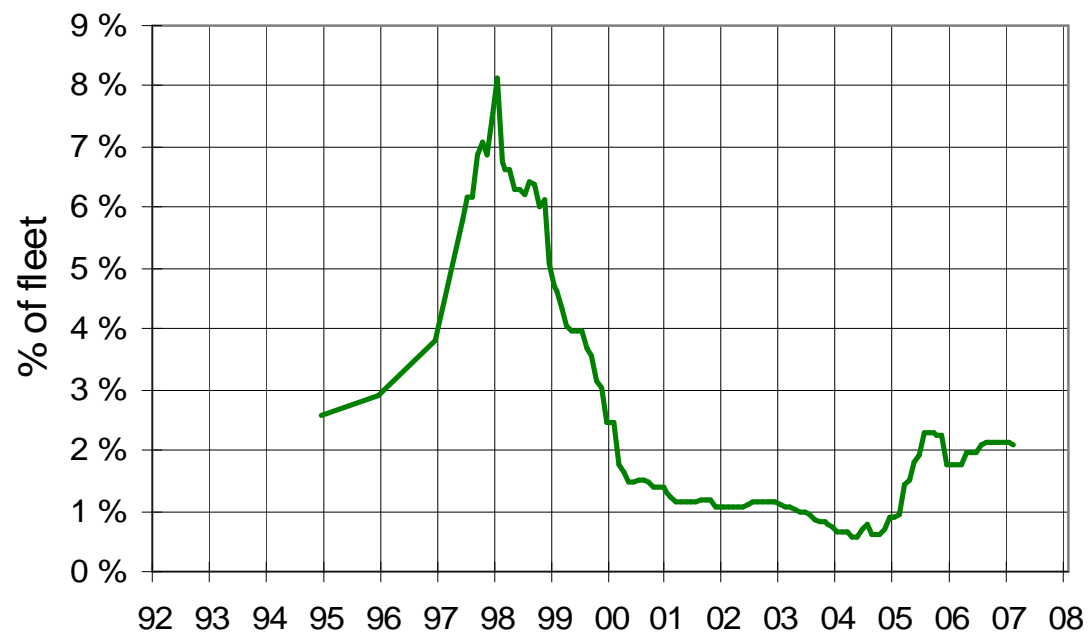
Reefer orderbook
